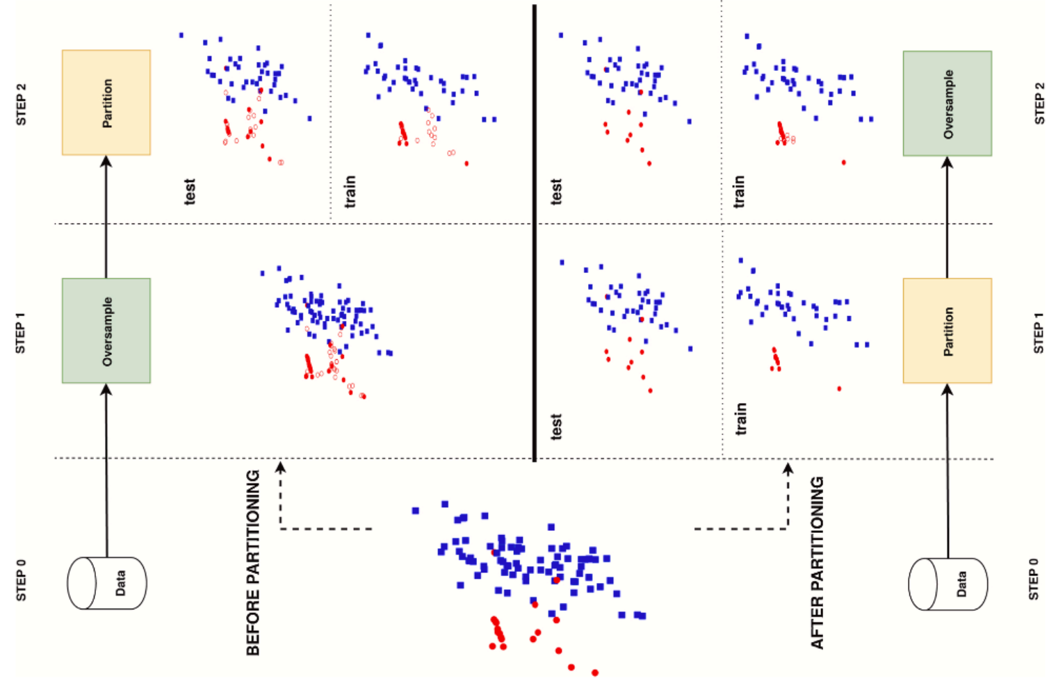
Fig. Comparing the impact of applying over-sampling prior to data partitioning to applying over-sampling after data partitioning on an artificial two-dimensional classification problem.
